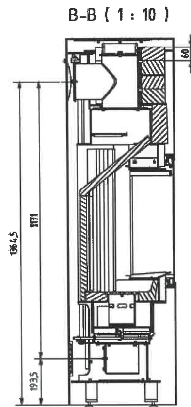
Massblatt Arto 155 / 175
