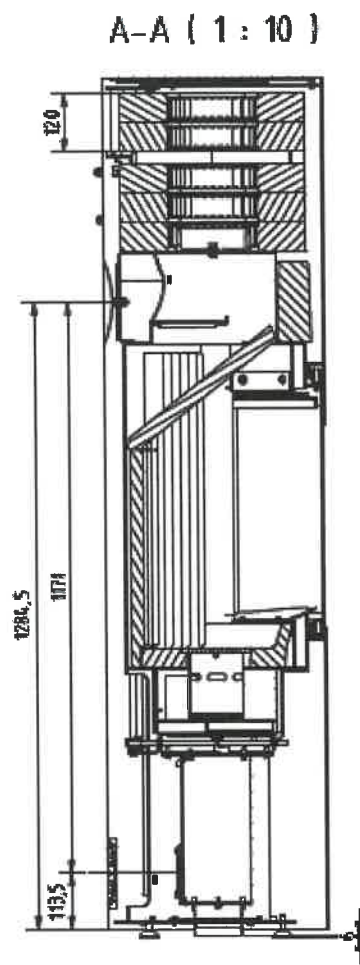
Massblatt Arto 155 / 175
